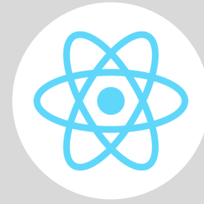
React
