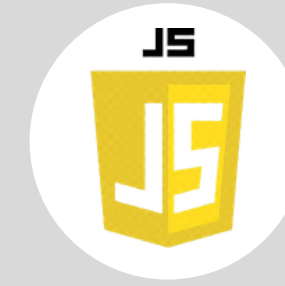
JavaScript
